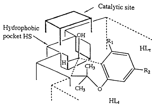
Figure 3. Reactive conformation of 4-hydroxy-2,2-dimethylchromans superimposed on the PFL active site (according to Naemura et al. 12 ).
